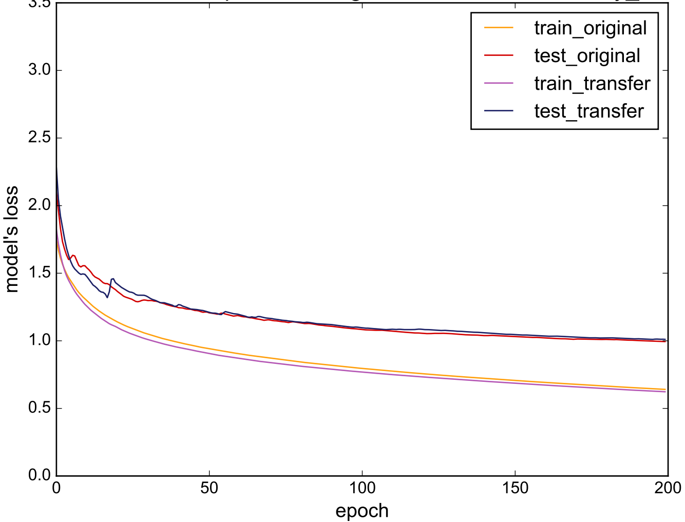
Source: Earthquakes - Target: uWaveGestureLibrary_Z
