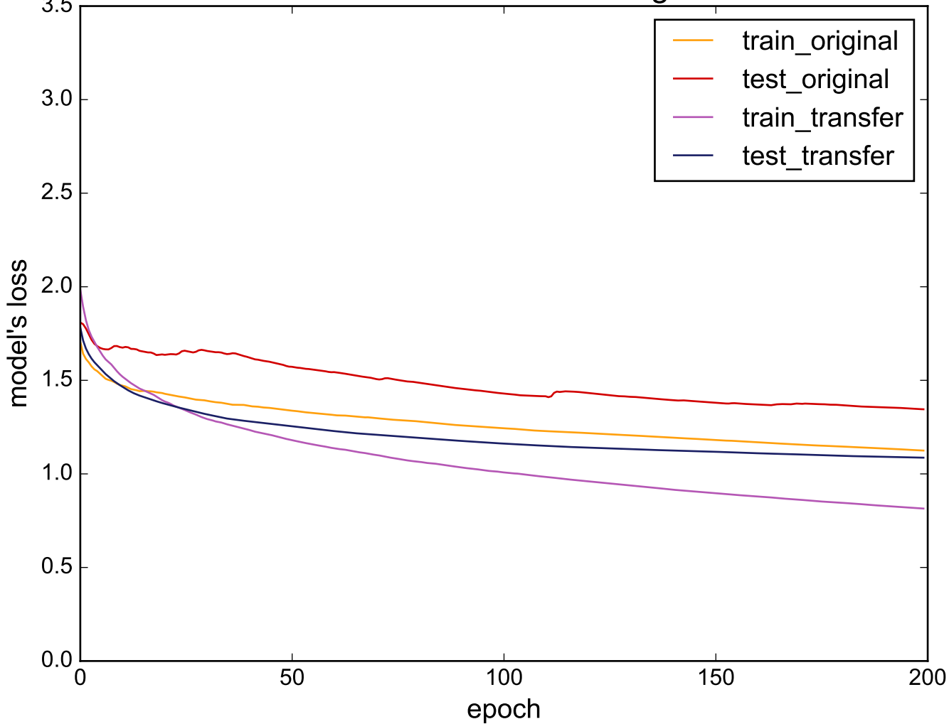
Source: ElectricDevices - Target: Beef
