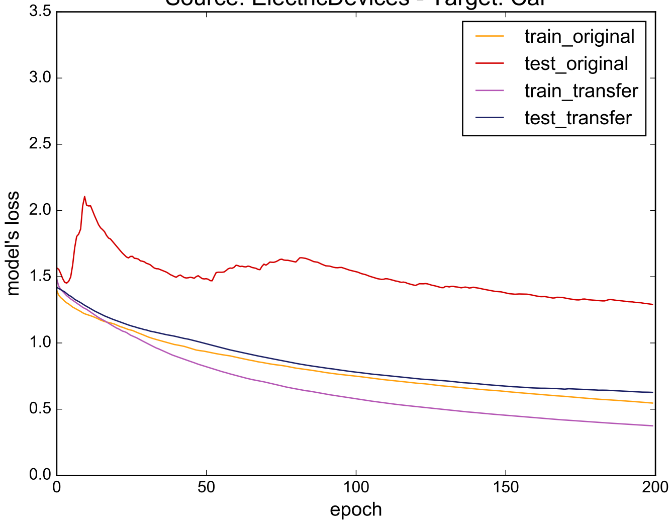
Source: ElectricDevices - Target: Car
