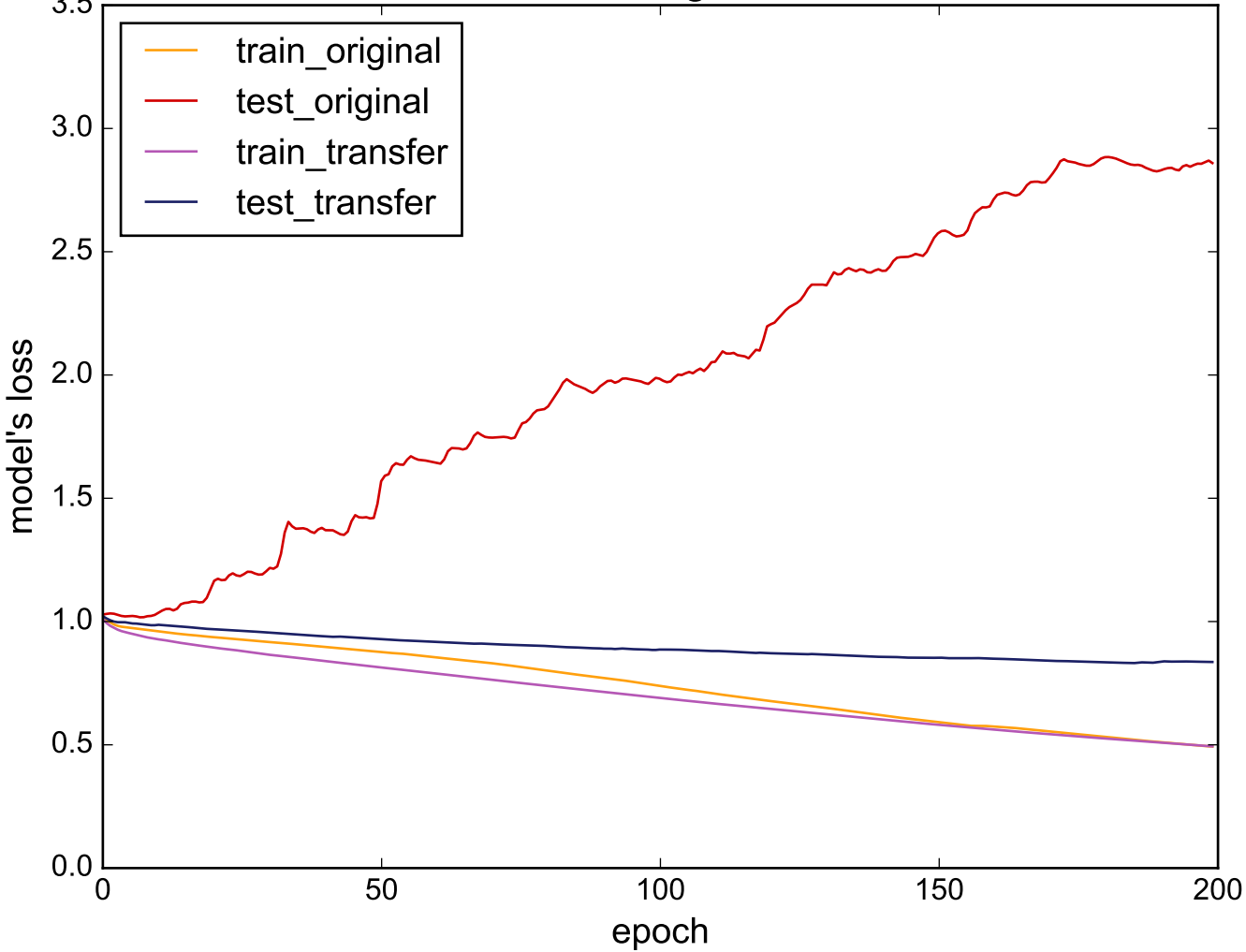
Source: ElectricDevices - Target: ChlorineConcentration
