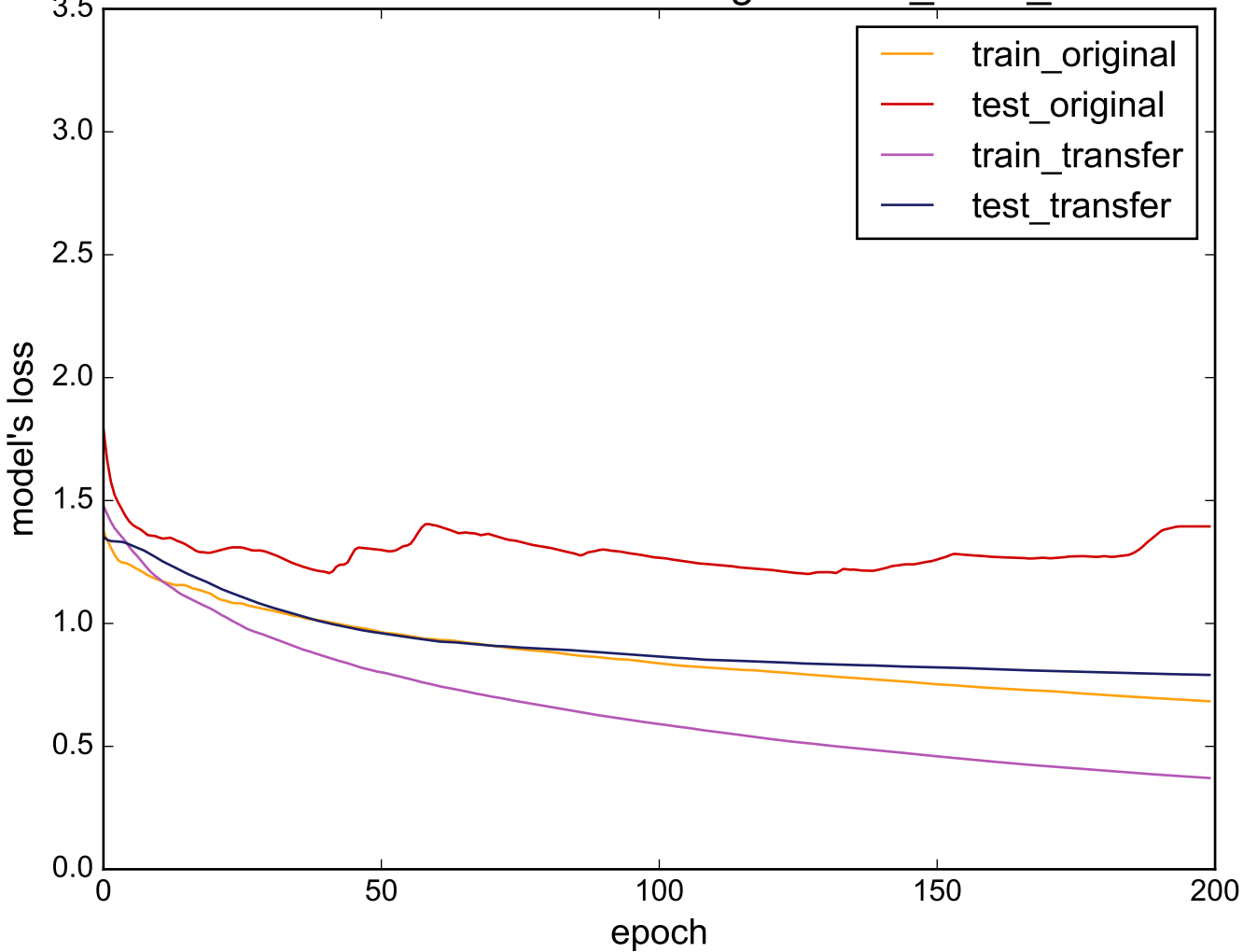
Source: ElectricDevices - Target: CinC_ECG_torso
