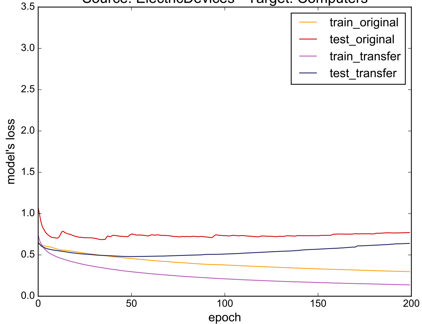
Source: ElectricDevices - Target: Computers
