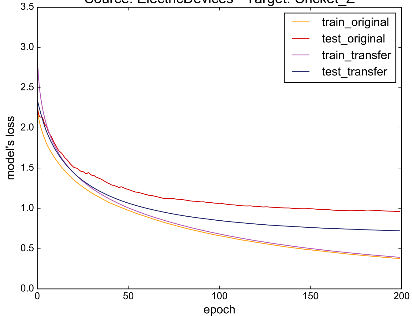
Source: ElectricDevices - Target: Cricket_Z
