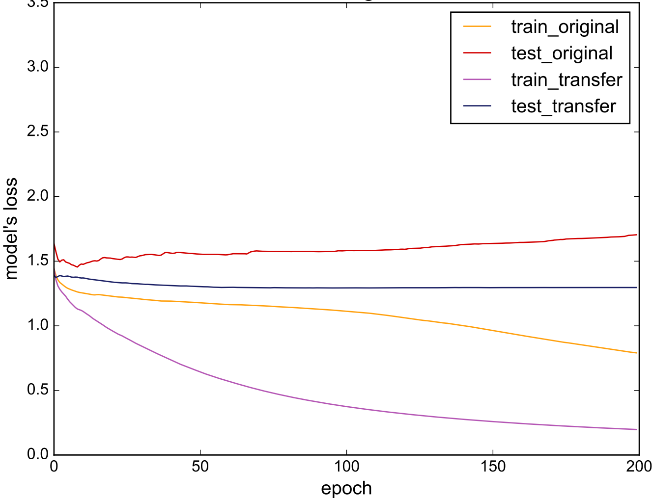
Source: ElectricDevices - Target: DiatomSizeReduction
