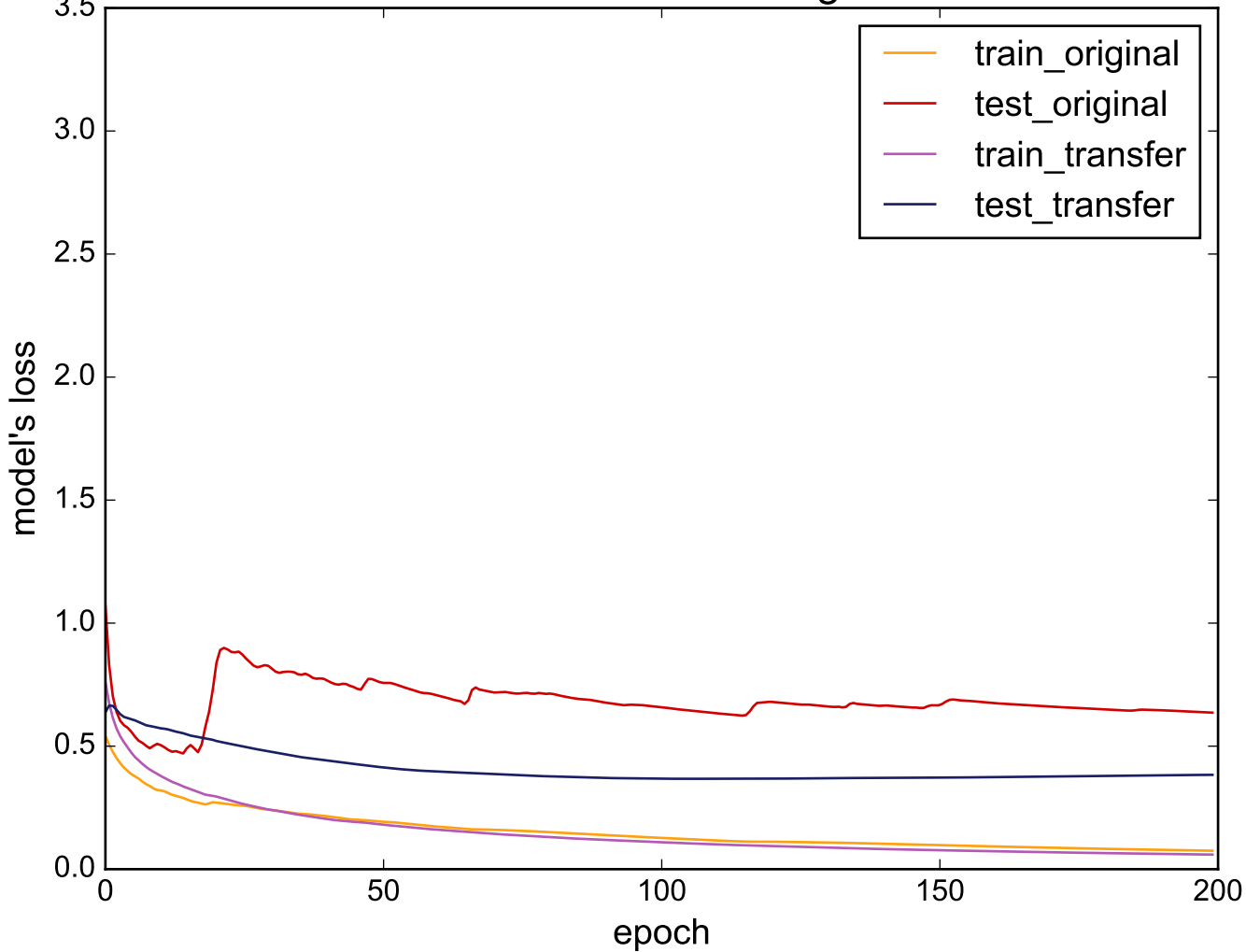
Source: ElectricDevices - Target: ECG200
