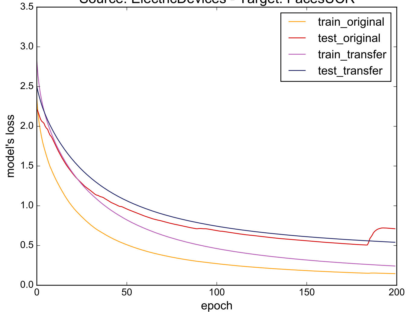
Source: ElectricDevices - Target: FacesUCR
