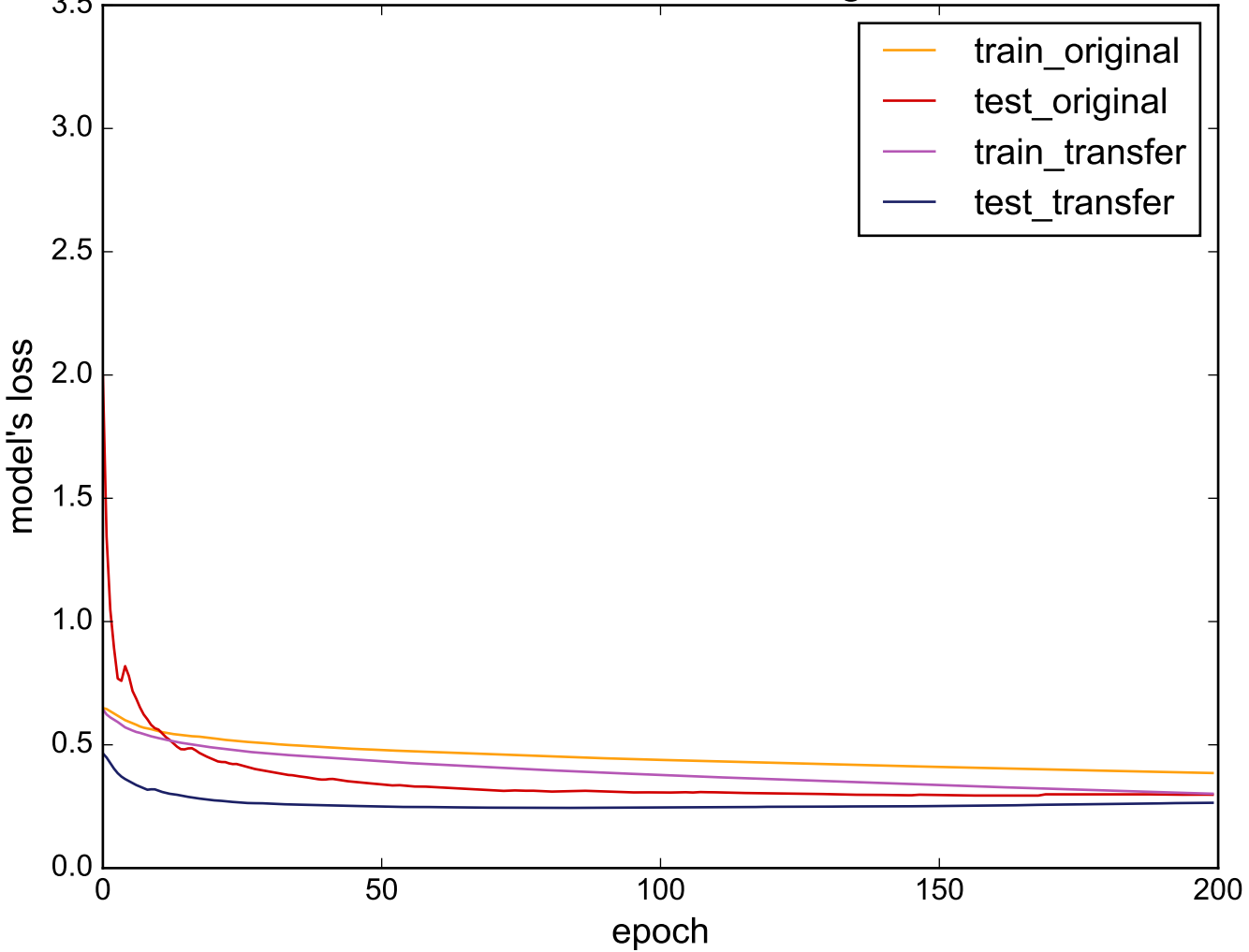
Source: ElectricDevices - Target: FordB
