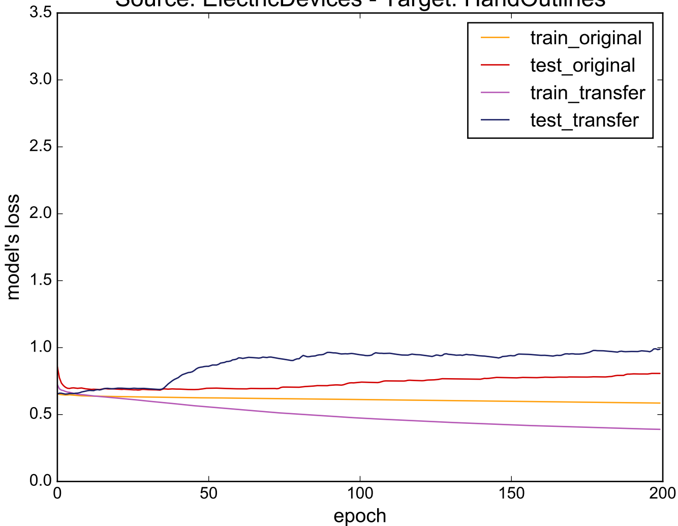
Source: ElectricDevices - Target: HandOutlines
