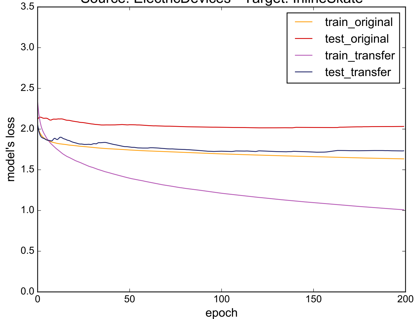
Source: ElectricDevices - Target: InlineSkate
