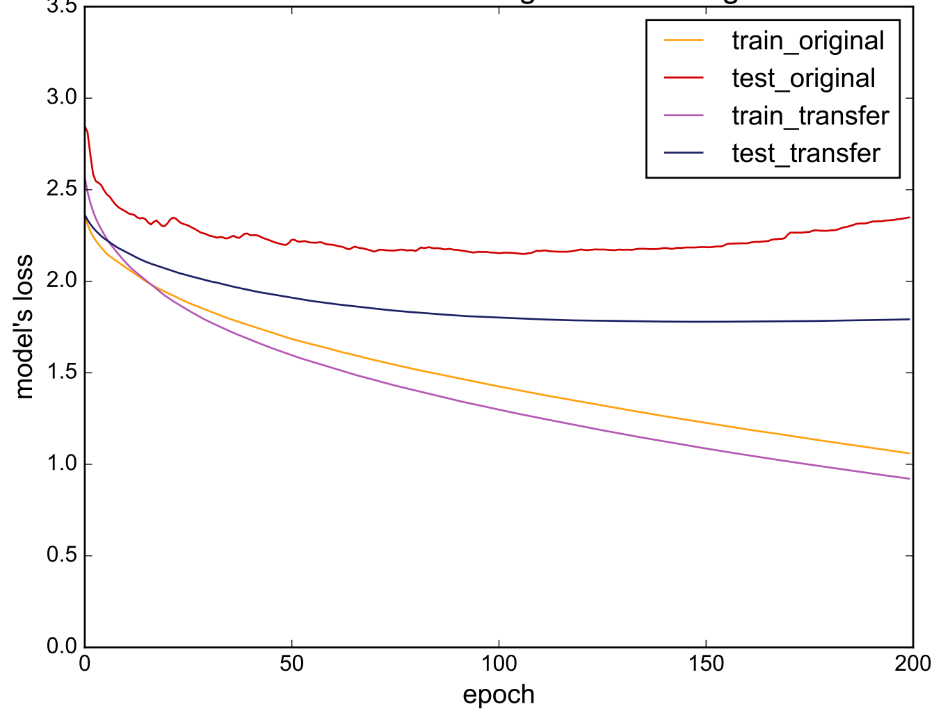
Source: ElectricDevices - Target: InsectWingbeatSound
