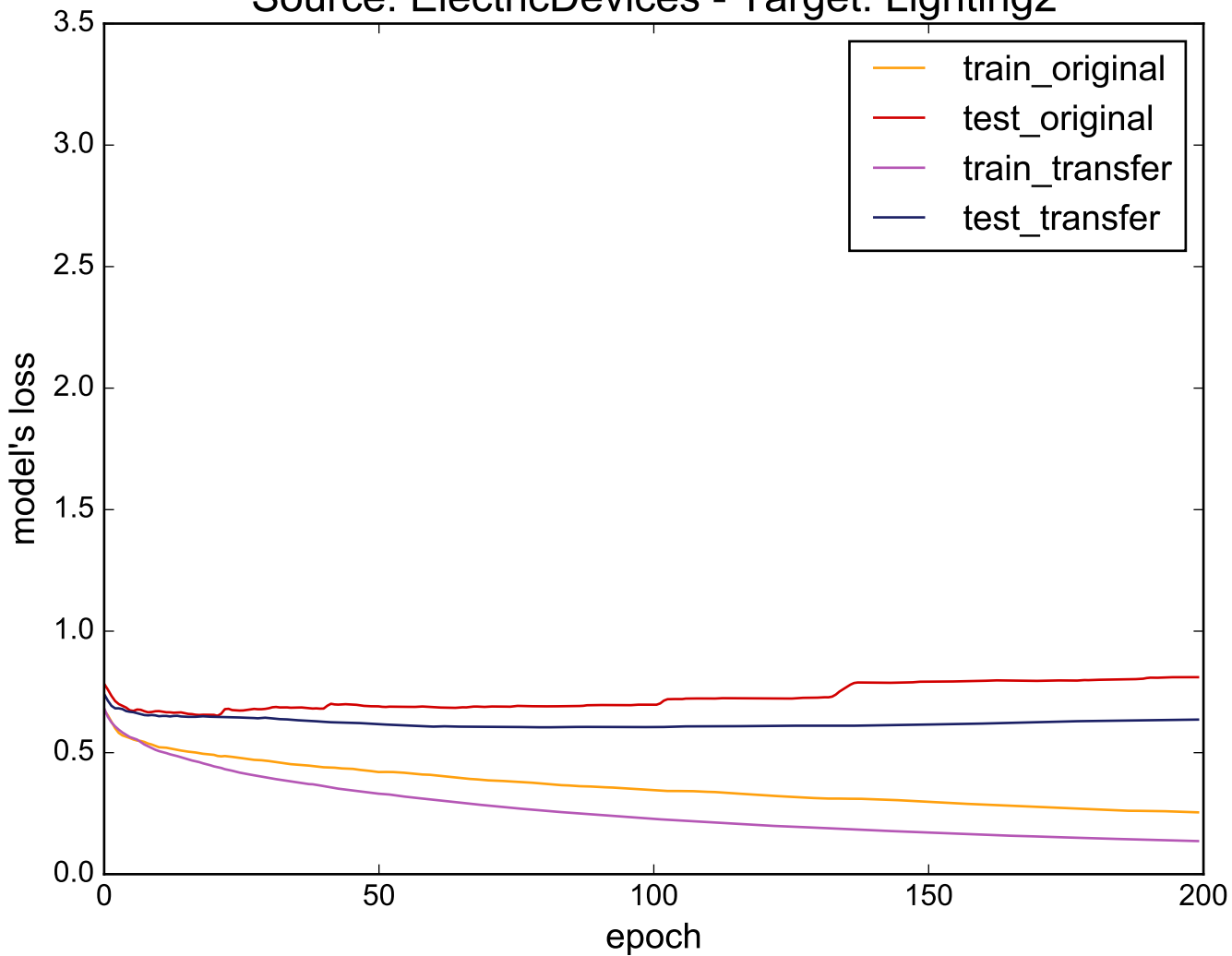
Source: ElectricDevices - Target: Lighting2
