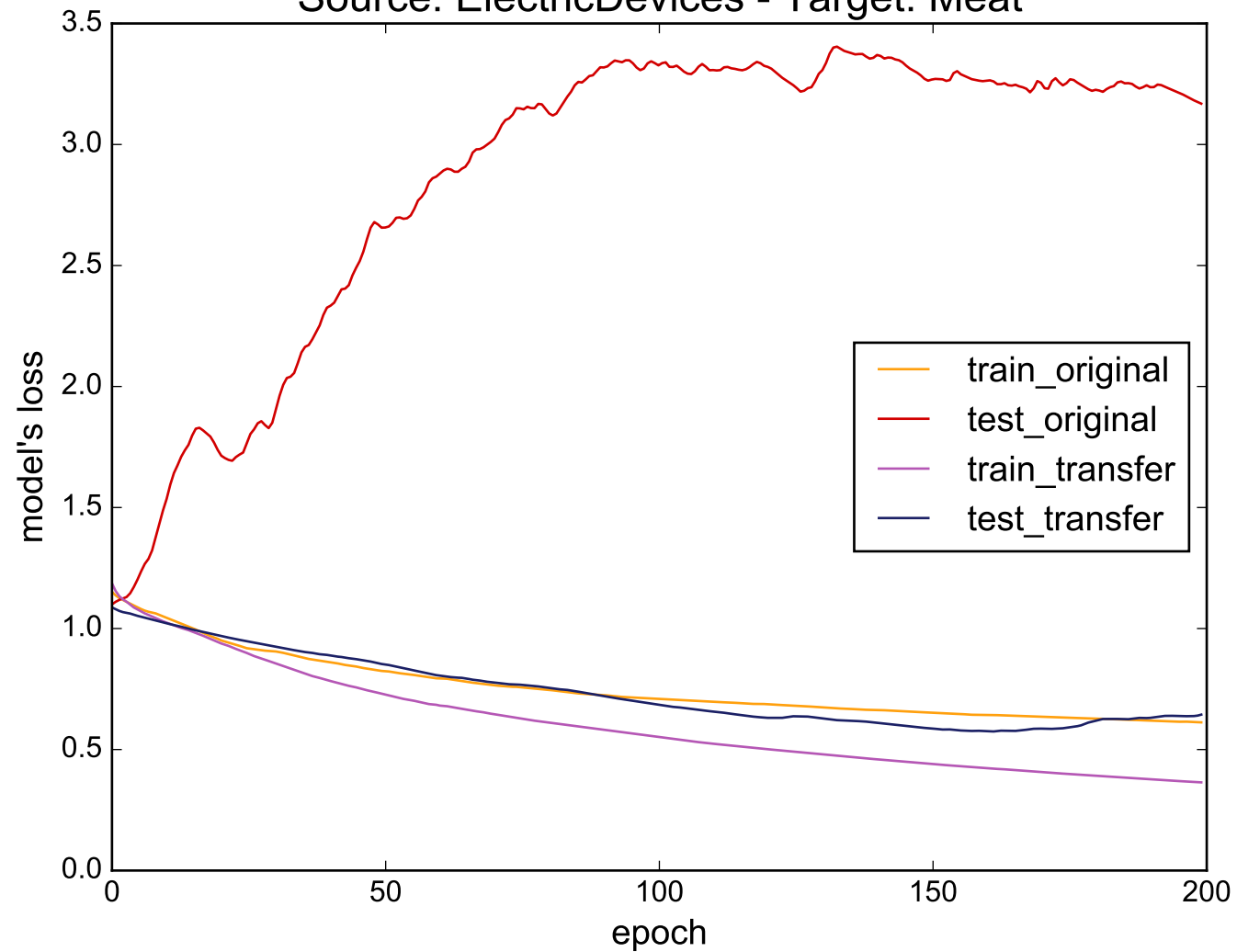
Source: ElectricDevices - Target: Meat
