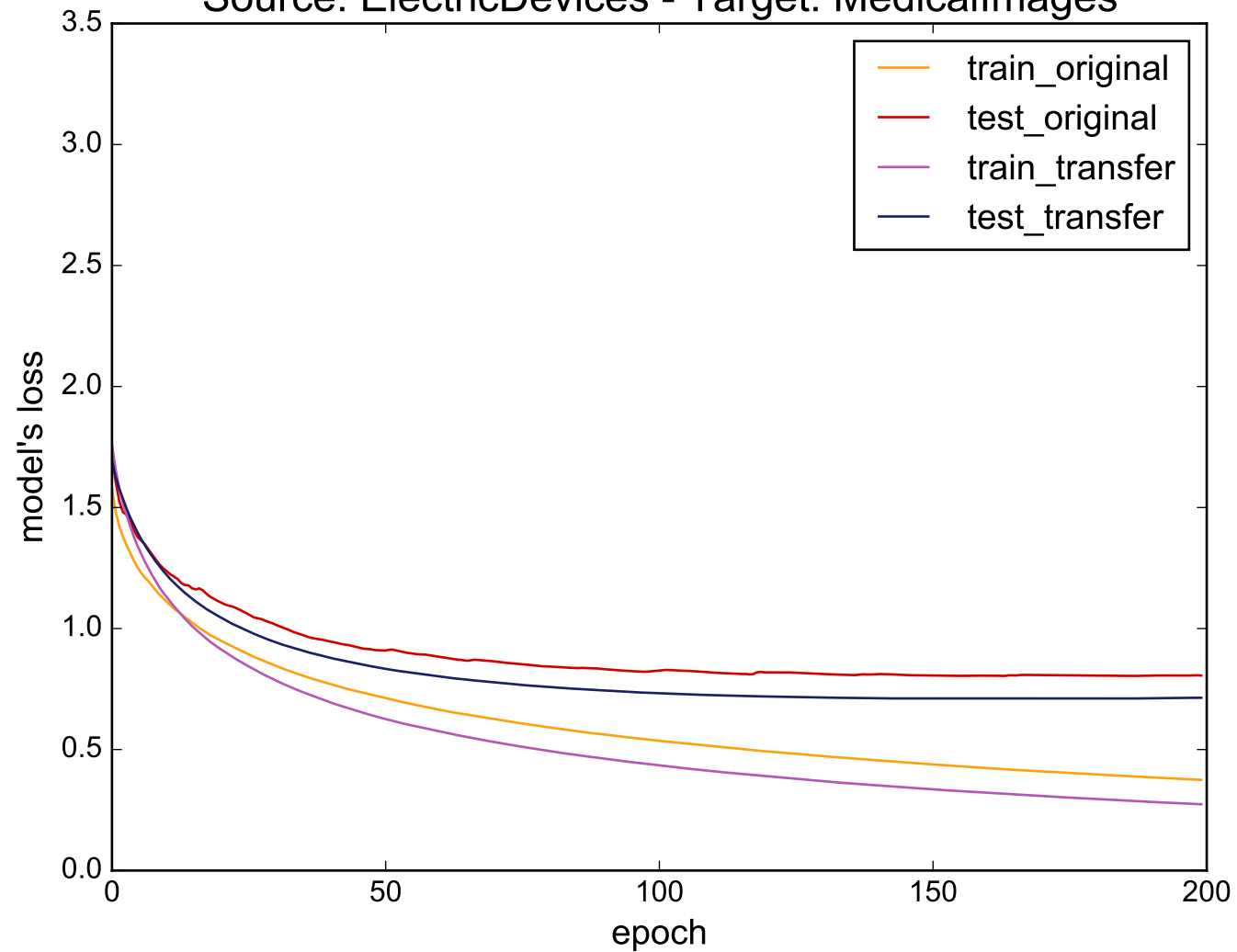
Source: ElectricDevices - Target: MedicalImages
