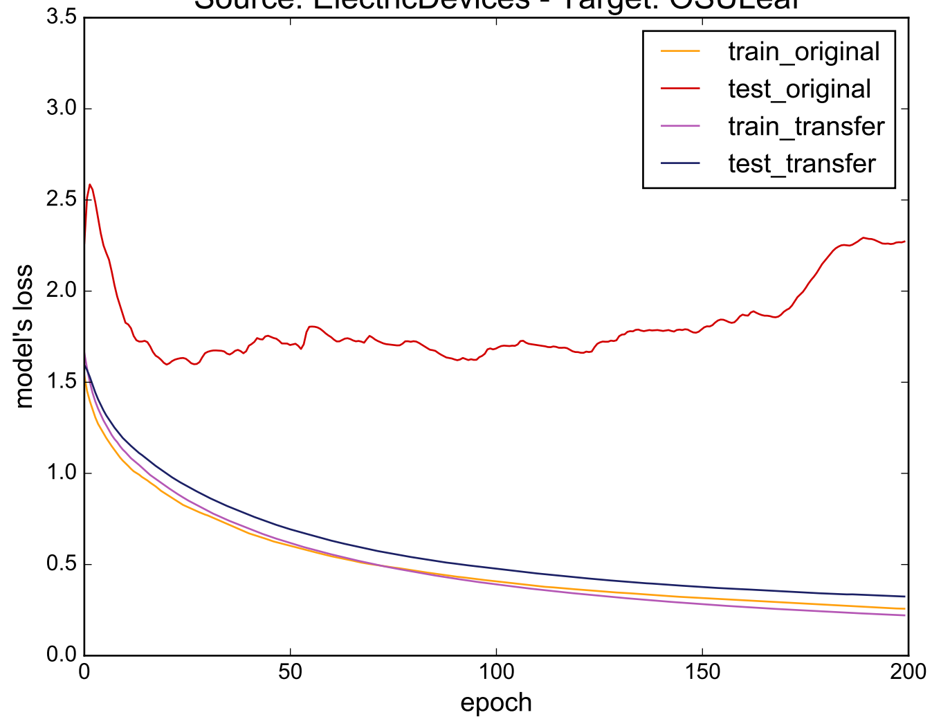
Source: ElectricDevices - Target: OSULeaf
