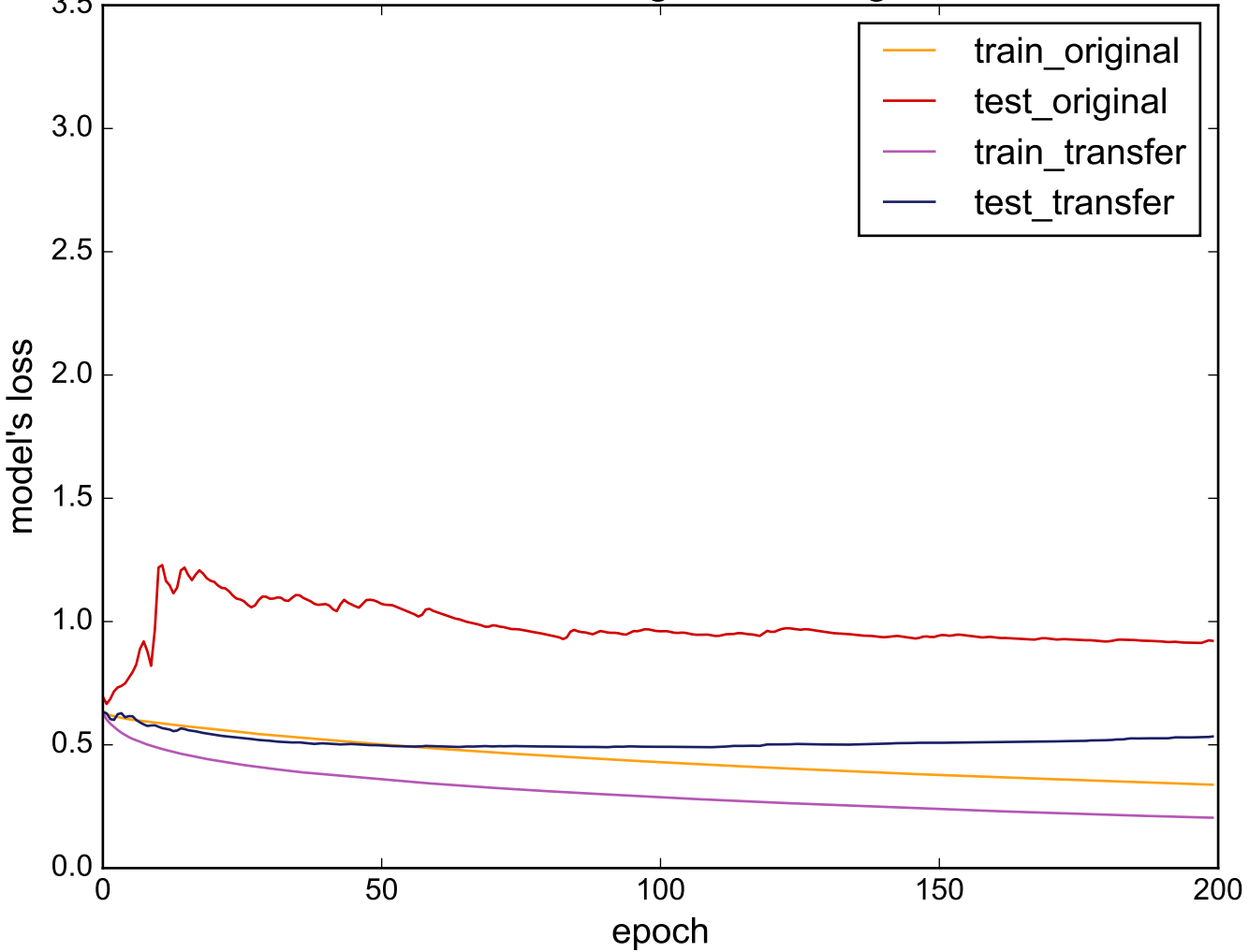
Source: ElectricDevices - Target: PhalangesOutlinesCorrect
