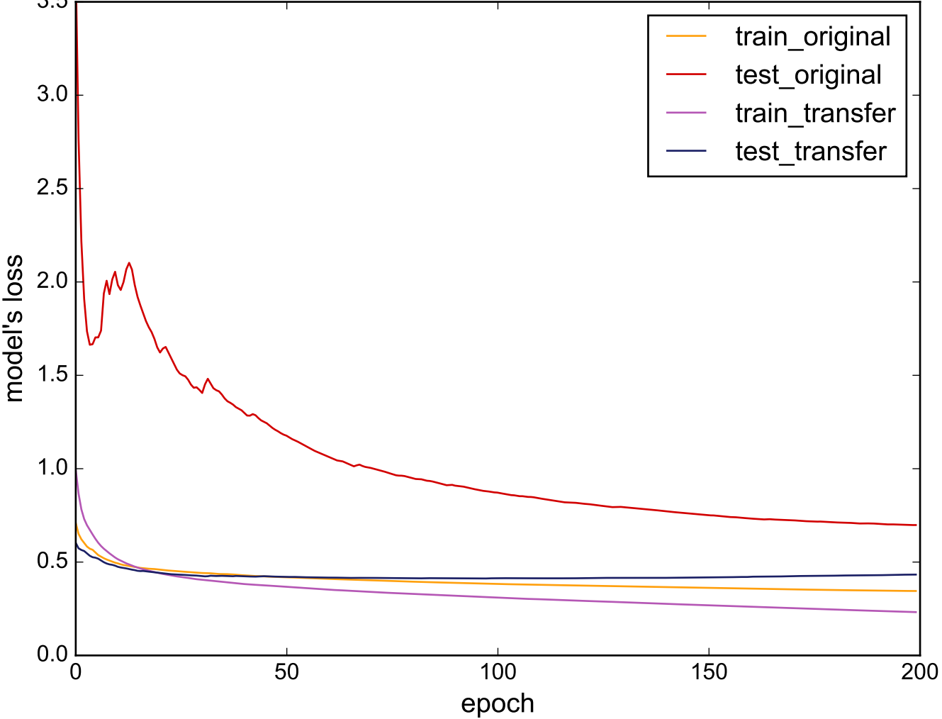
Source: ElectricDevices - Target: ProximalPhalanxOutlineAgeGroup
