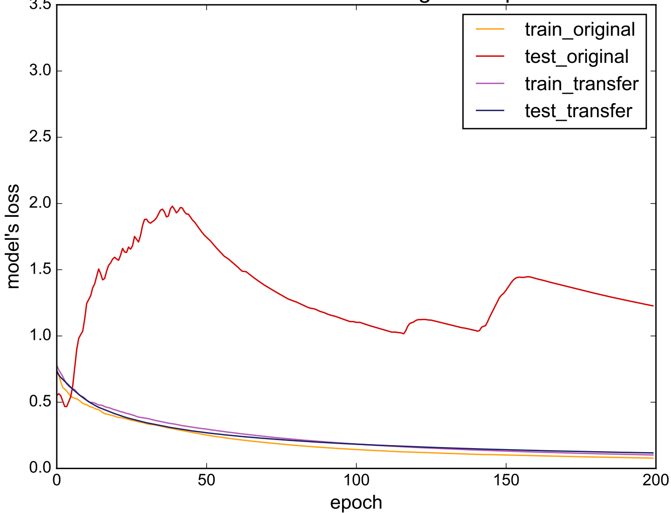
Source: ElectricDevices - Target: ShapeletSim
