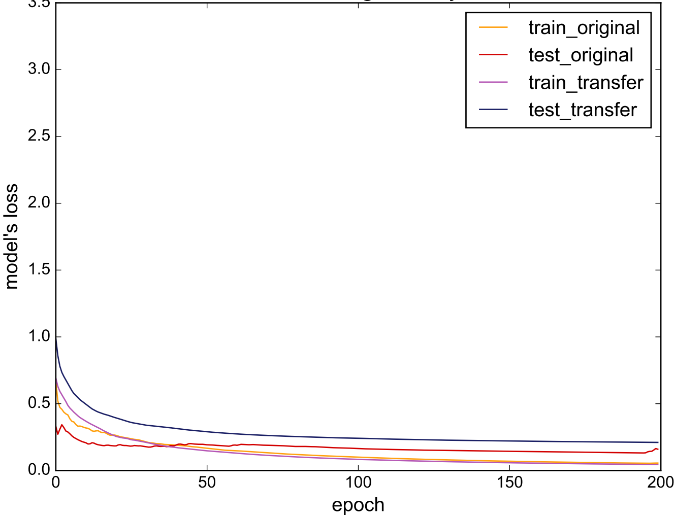
Source: ElectricDevices - Target: SonyAIBORobotSurface
