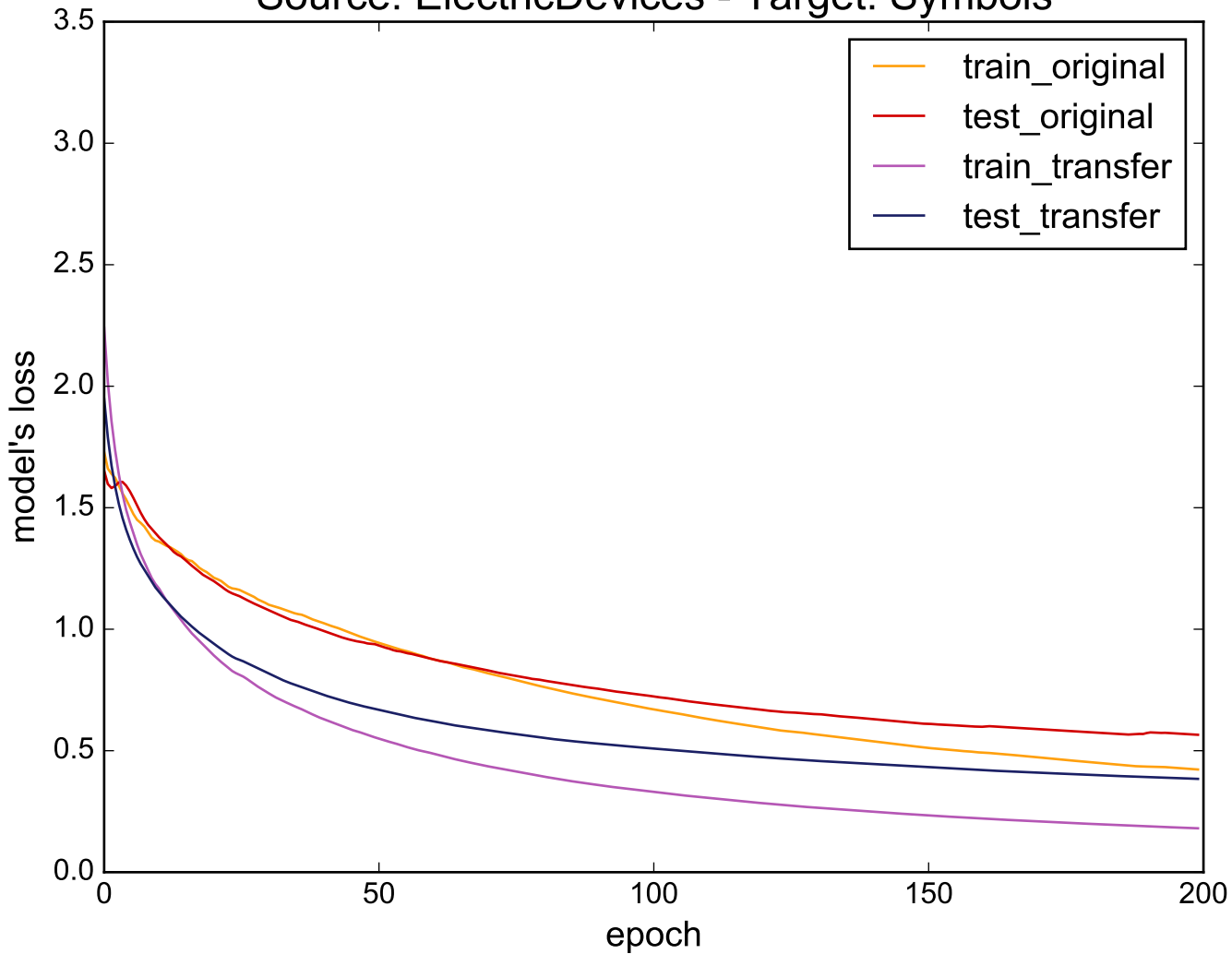
Source: ElectricDevices - Target: Symbols
