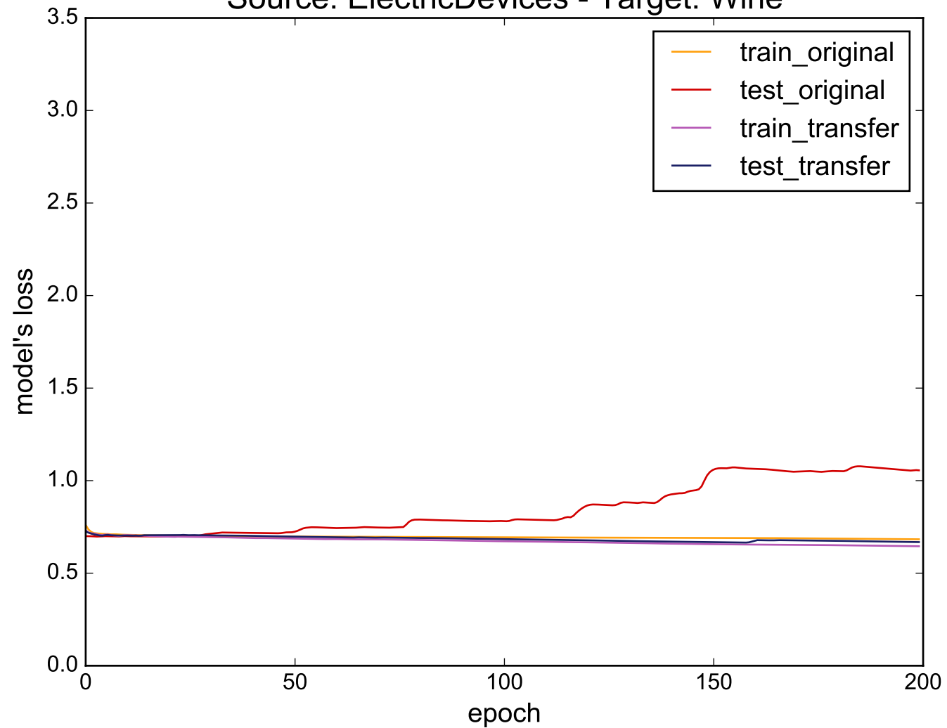
Source: ElectricDevices - Target: Wine
