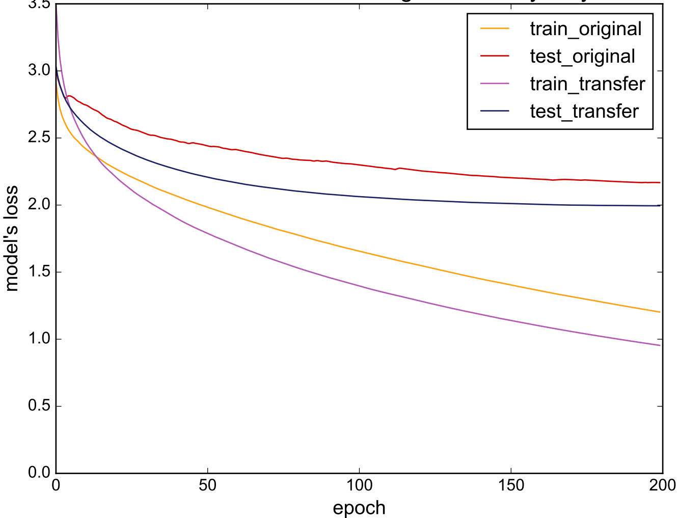
Source: ElectricDevices - Target: WordsSynonyms
