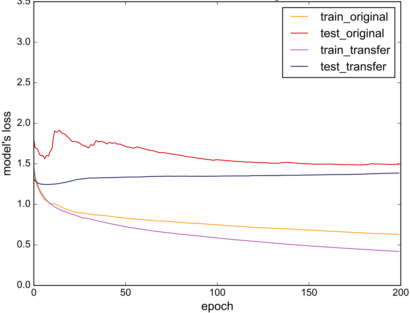
Source: ElectricDevices - Target: Worms
