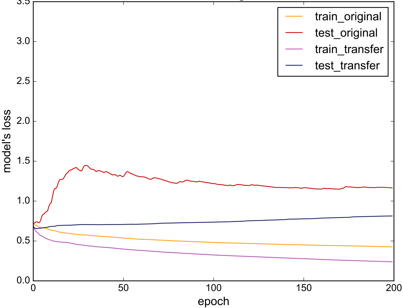
Source: ElectricDevices - Target: WormsTwoClass
