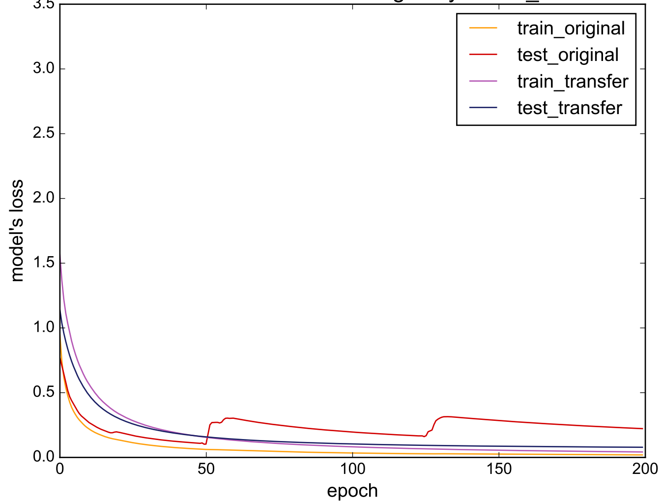
Source: ElectricDevices - Target: synthetic_control
