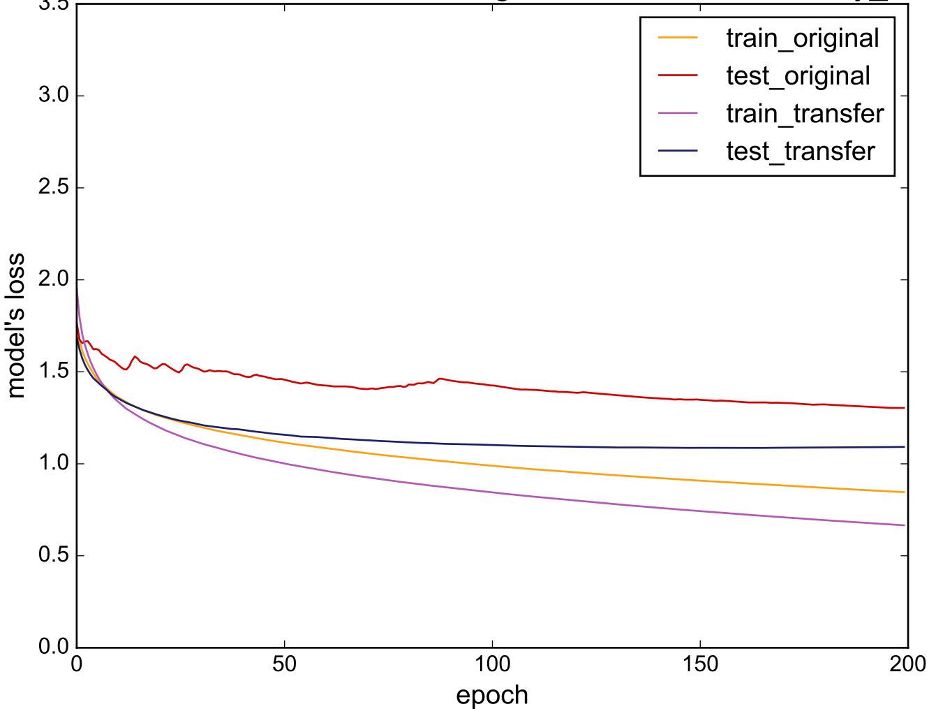
Source: ElectricDevices - Target: uWaveGestureLibrary_Y
