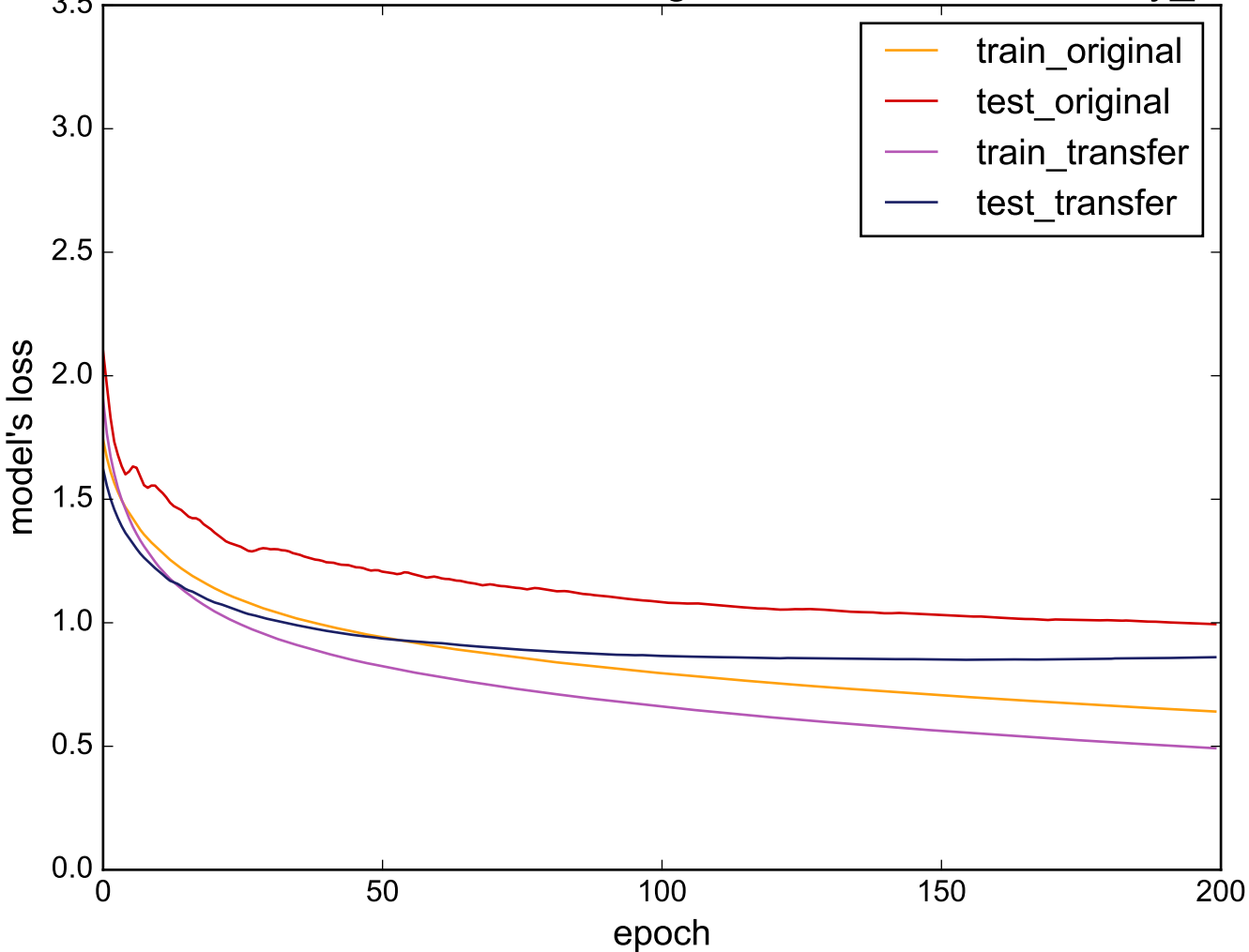
Source: ElectricDevices - Target: uWaveGestureLibrary_Z
