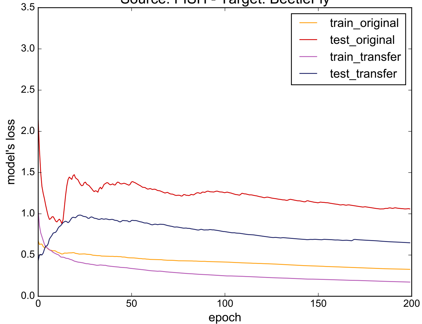
Source: FISH - Target: BeetleFly
