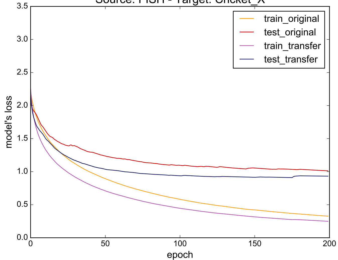
Source: FISH - Target: Cricket_X
