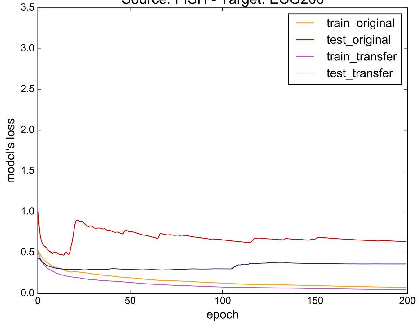
Source: FISH - Target: ECG200
