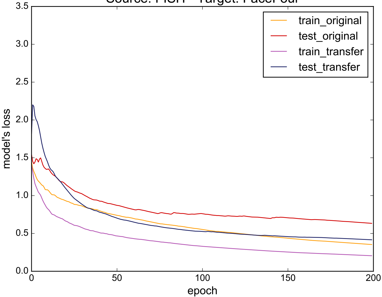
Source: FISH - Target: FaceFour
