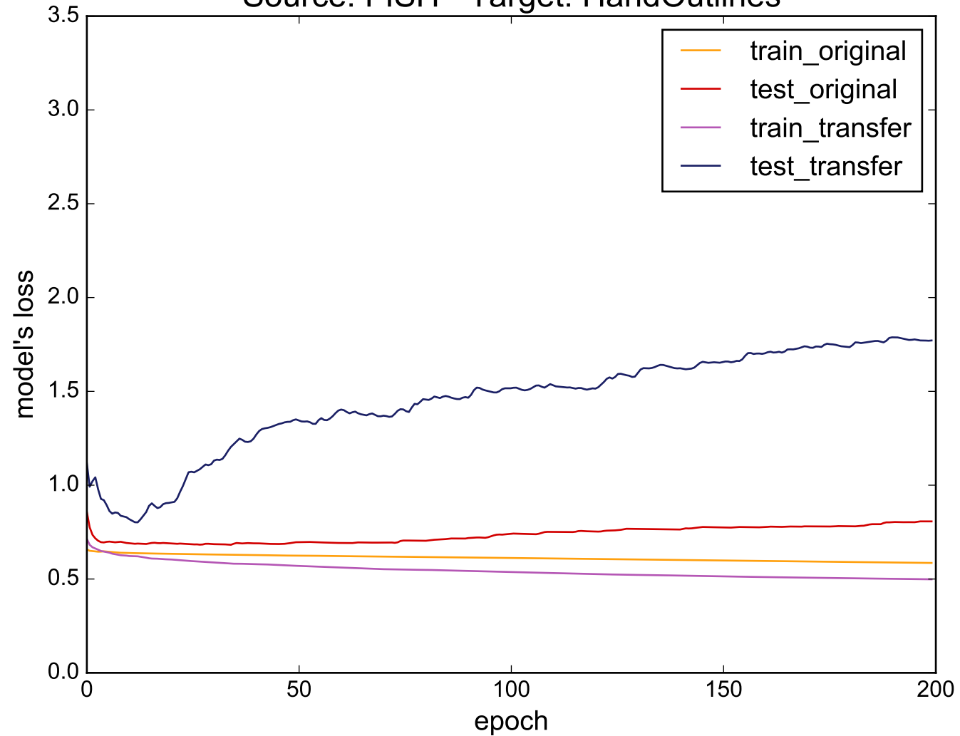
Source: FISH - Target: HandOutlines
