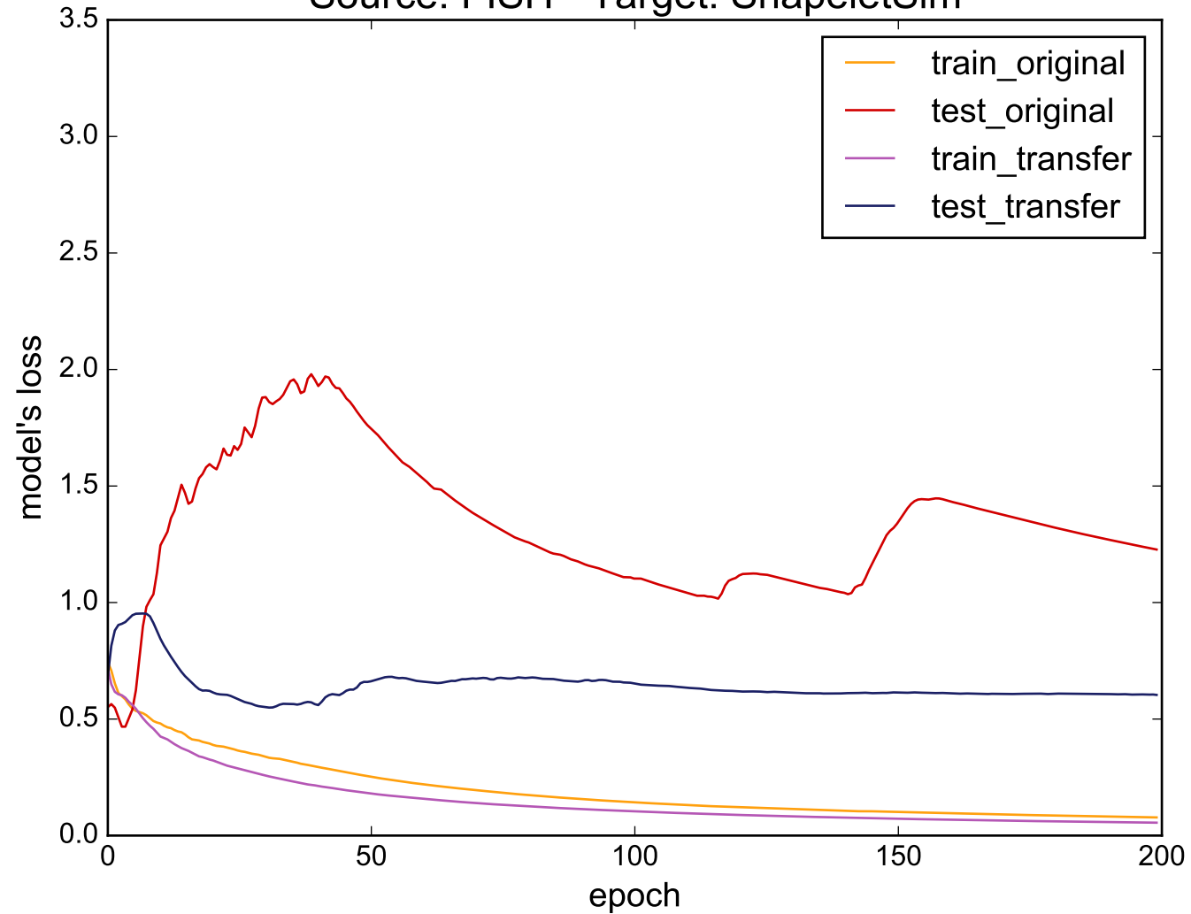
Source: FISH - Target: ShapeletSim
