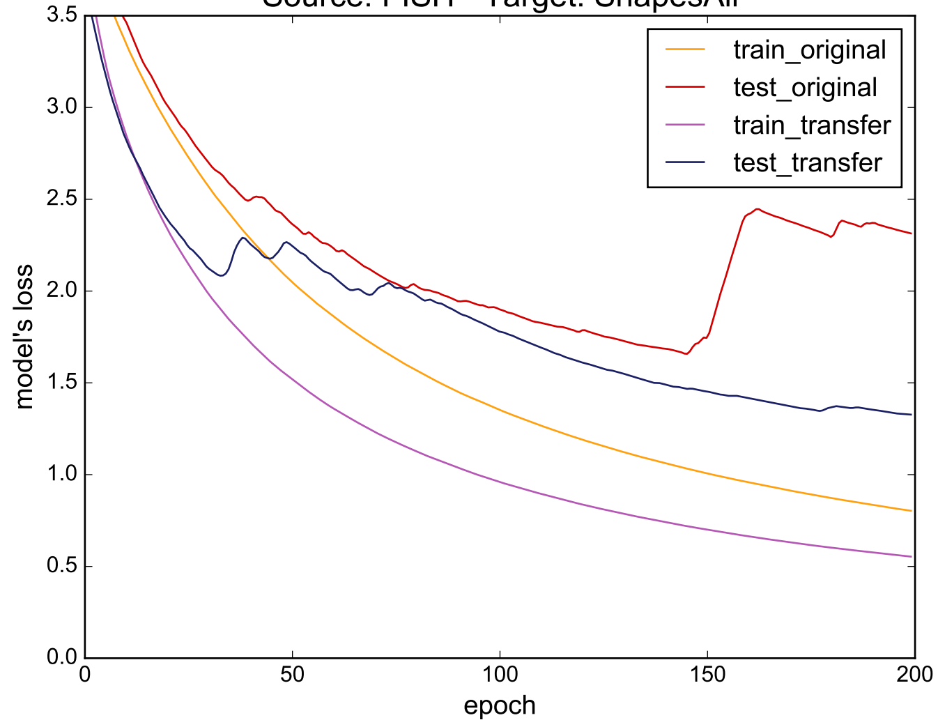
Source: FISH - Target: ShapesAll
