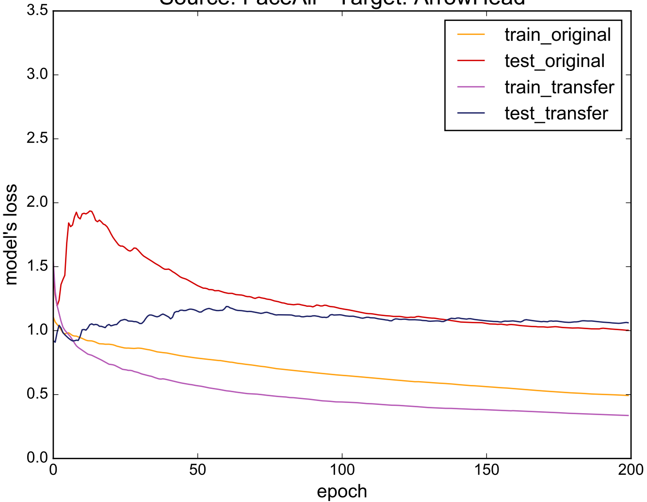
Source: FaceAll - Target: ArrowHead
