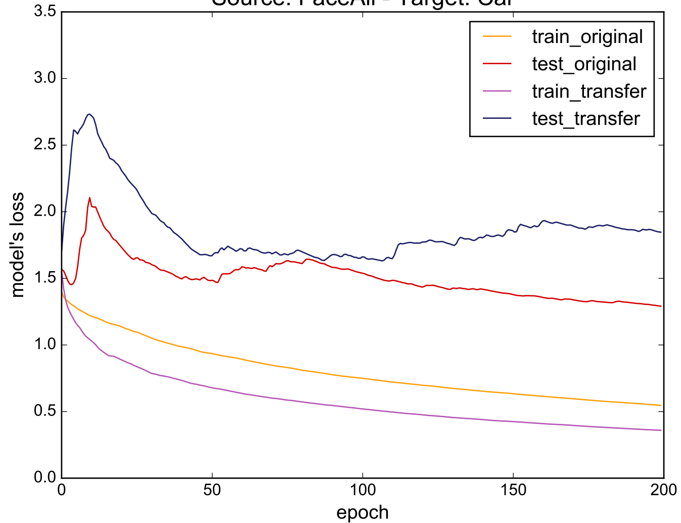
Source: FaceAll - Target: Car
