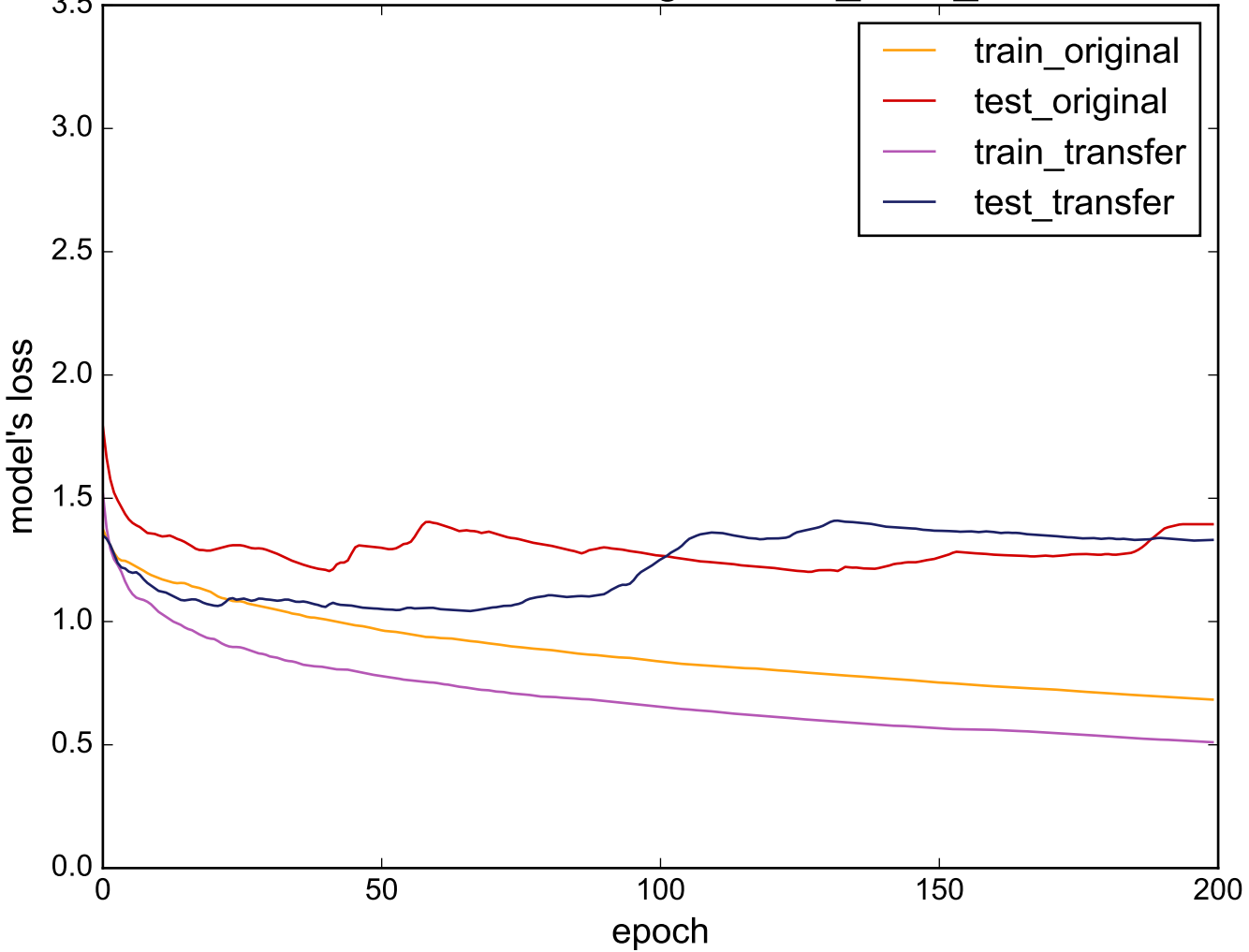
Source: FaceAll - Target: CinC_ECG_torso
