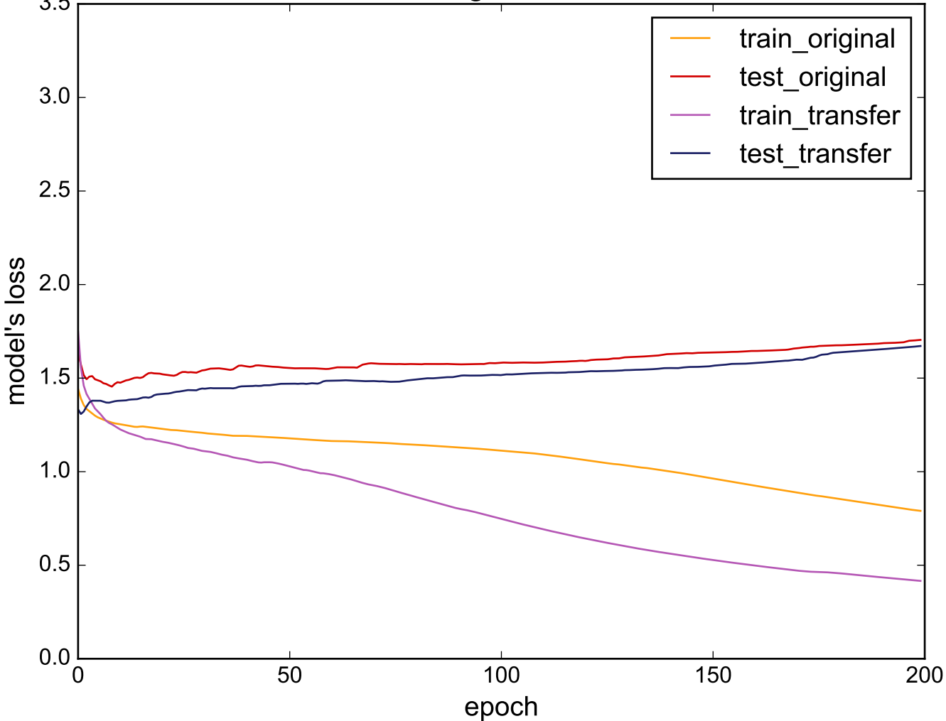
Source: FaceAll - Target: DiatomSizeReduction
