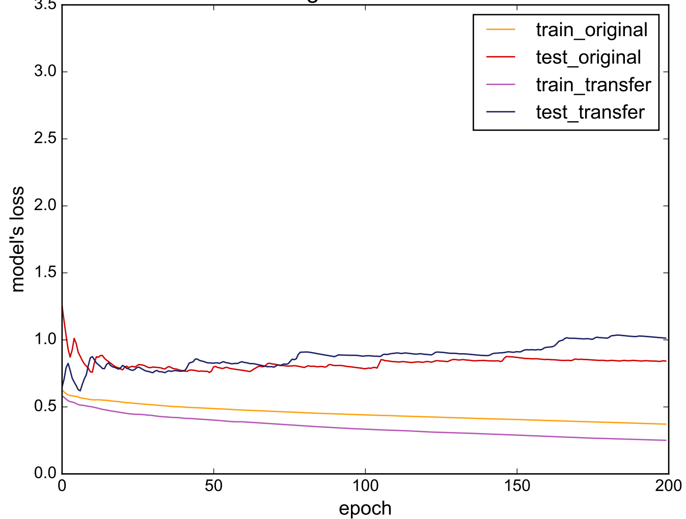
Source: FaceAll - Target: DistalPhalanxOutlineCorrect
