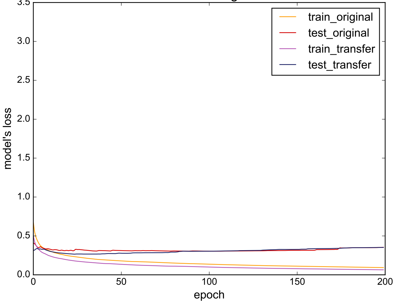
Source: FaceAll - Target: ECG5000
