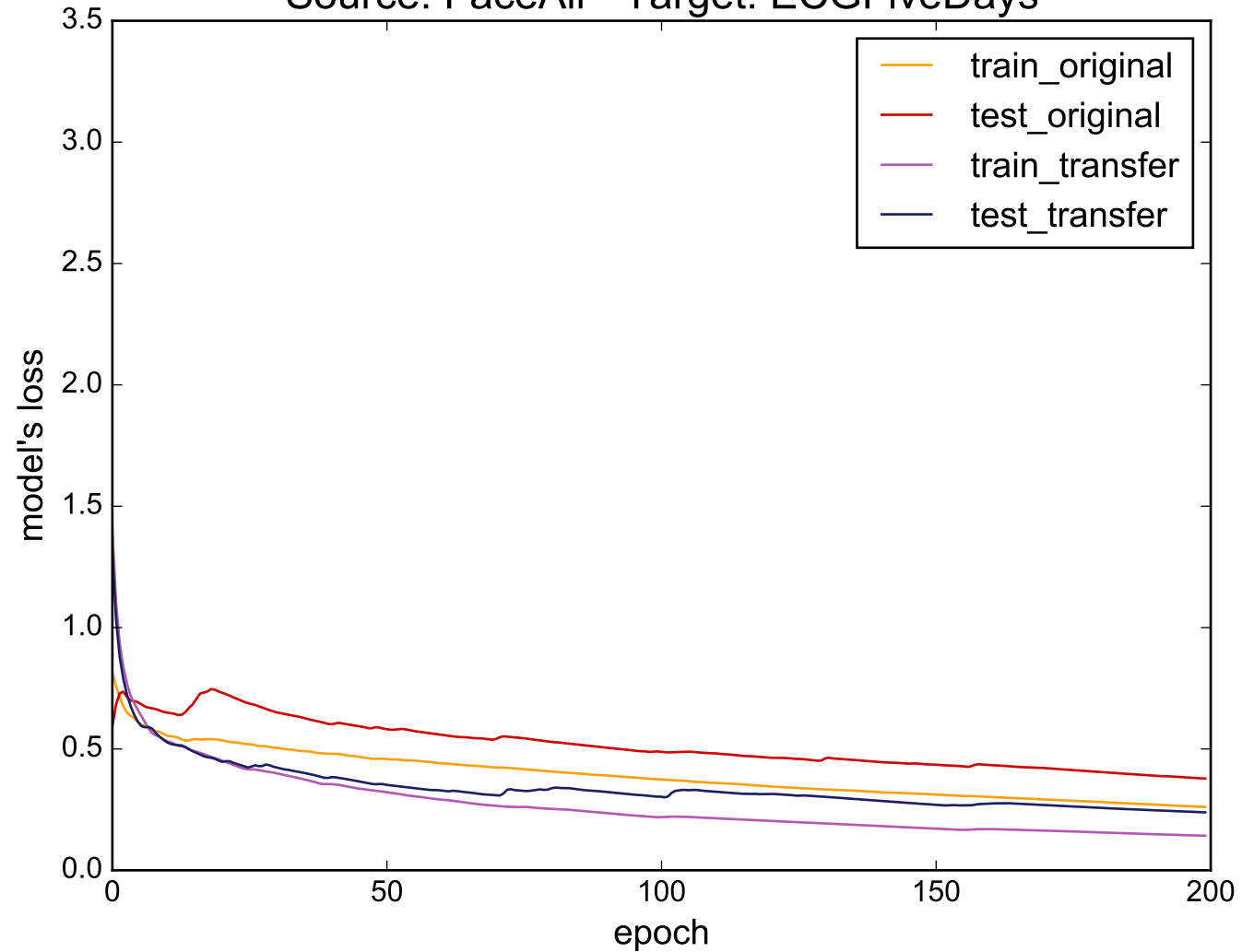
Source: FaceAll - Target: ECGFiveDays
