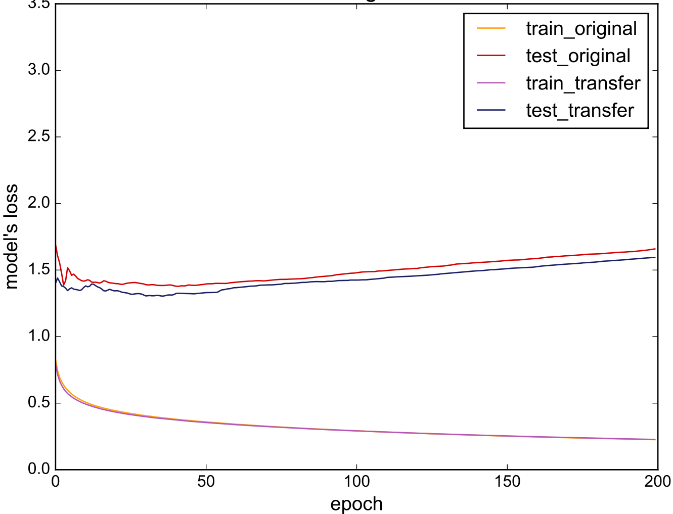
Source: FaceAll - Target: ElectricDevices
