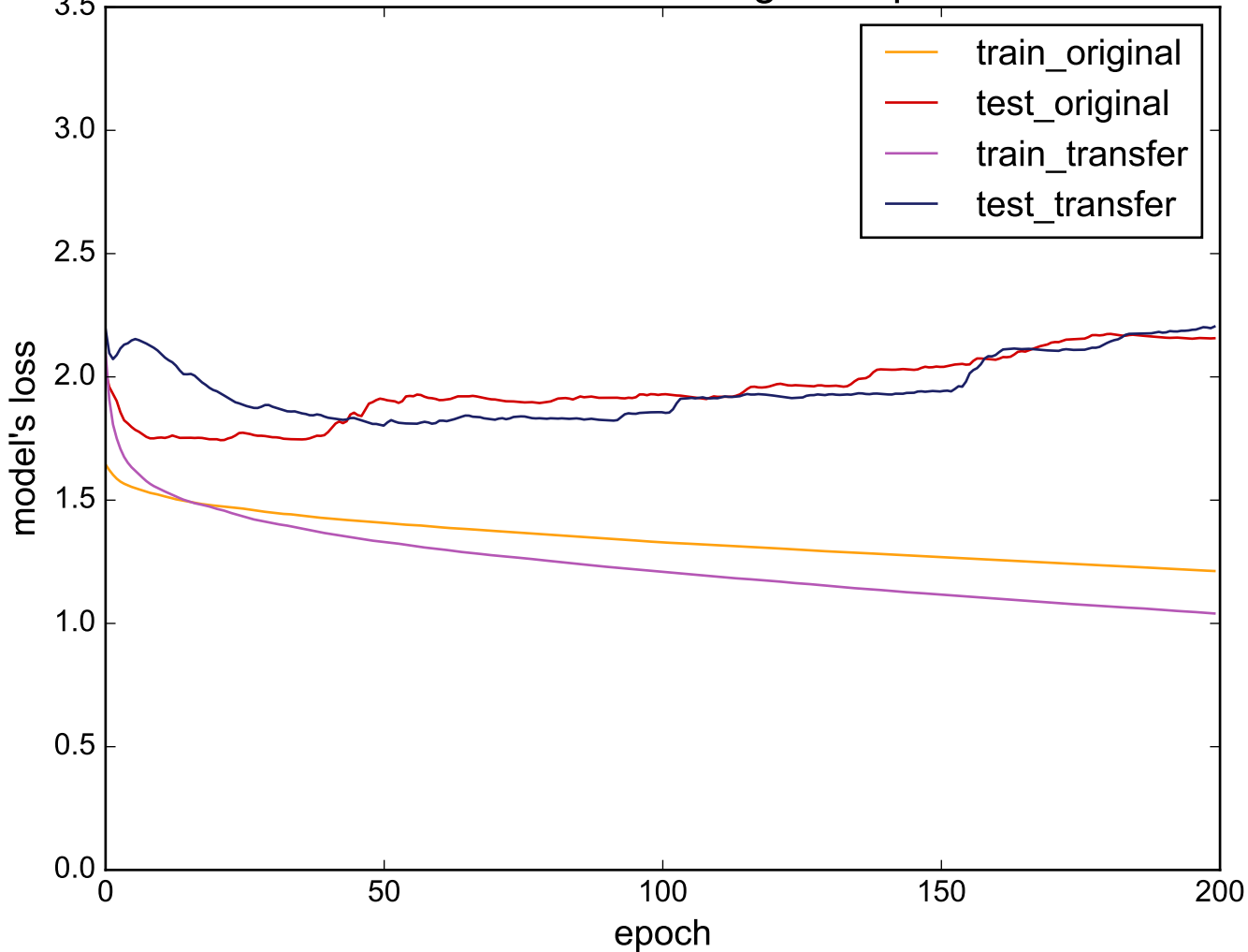
Source: FaceAll - Target: Haptics
