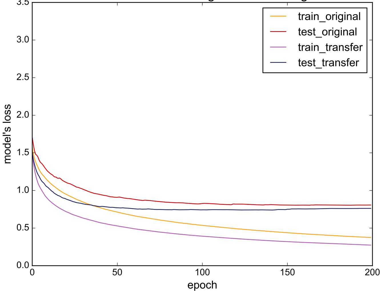
Source: FaceAll - Target: MedicalImages
