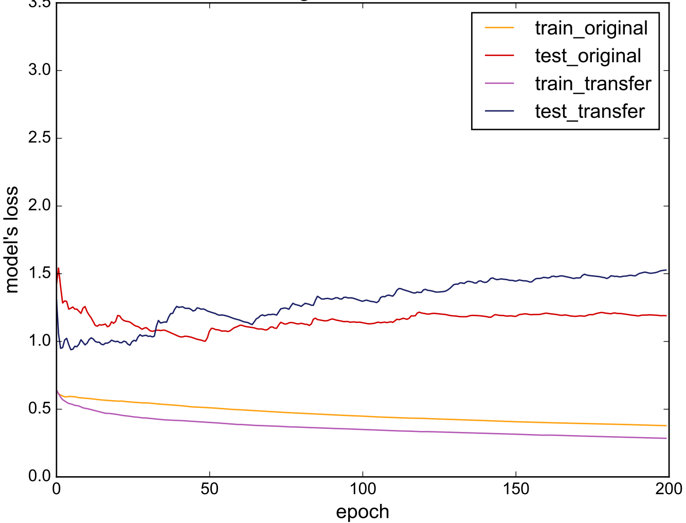
Source: FaceAll - Target: MiddlePhalanxOutlineCorrect
