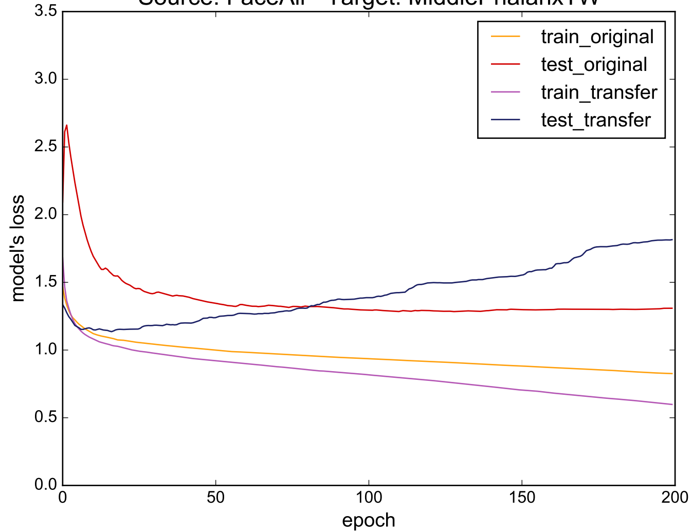
Source: FaceAll - Target: MiddlePhalanxTW
