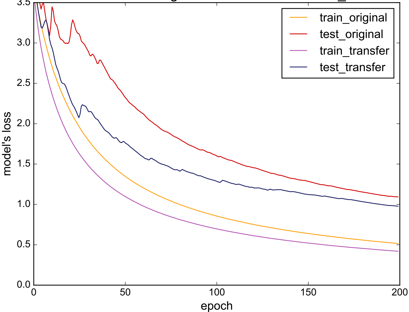
Source: FaceAll - Target: NonInvasiveFetalECG_Thorax1
